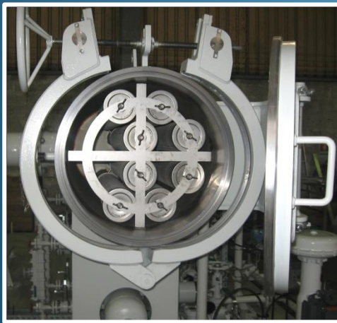
34" # 150 – HORIZONTAL "V" TYPE
