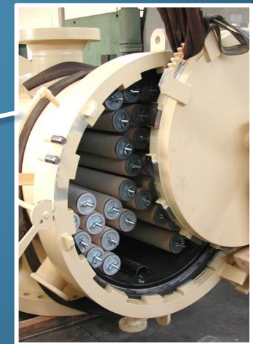
FCV TYPE - 39" # 600
