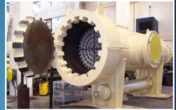
FILTER SEPARATOR FSO TYPE - 60" # 900, THK 82 mm
