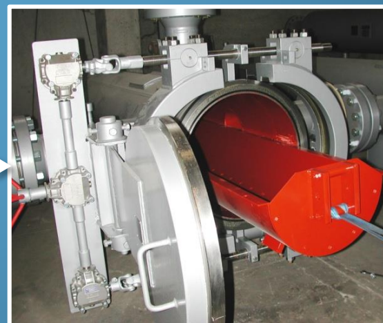
BIDIRECTIONAL TRAP 22" x 16" # 600
