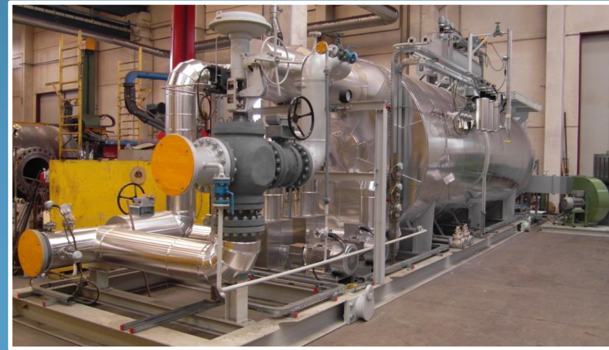
4 FORCED DRAFT OIL BATH HEATERS – 5.500.000 KCAL/h each OIL BATH TEMP. 220° C – OUTPUT GAS TEMP. 126.7° C
